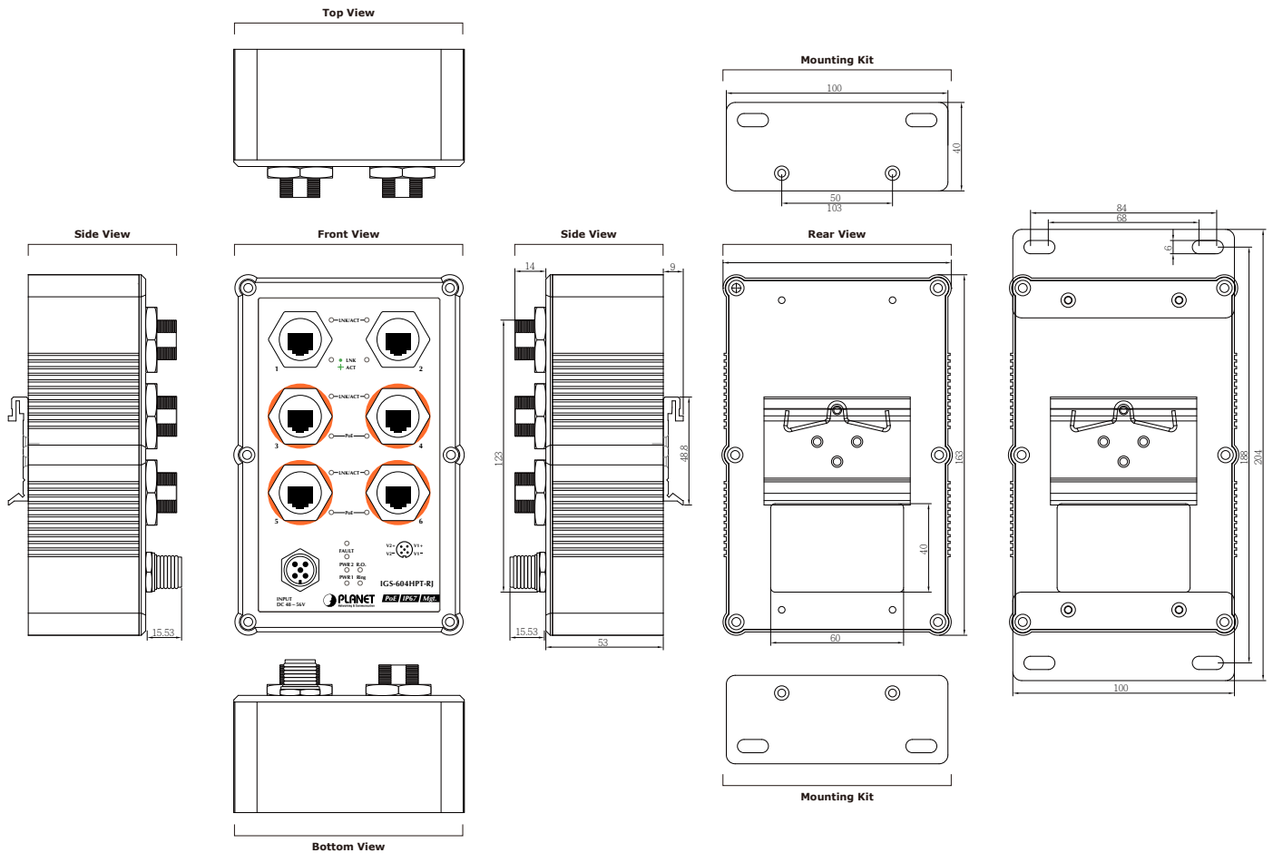
Dimensions ( unit = mm )
